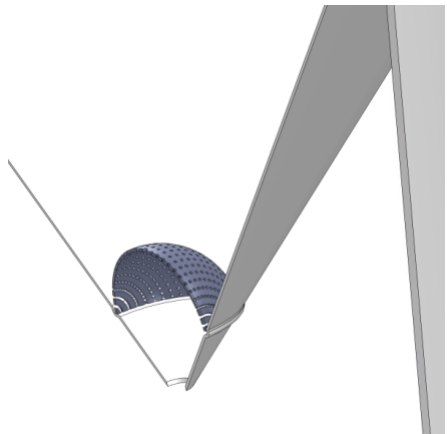
New anti-clogging system with large hole of 10mm diameter allowing water free falling on two new large spoons (cross section)
