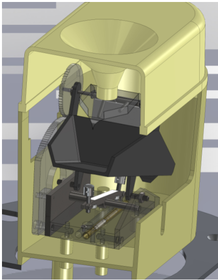
Rain-gauge mechanism (cross section)
